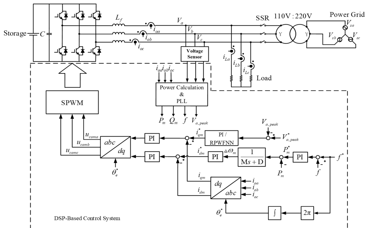
Control Block of Intelligent Control of Grid-Connected Microgrid with Virtual Inertia [13]
